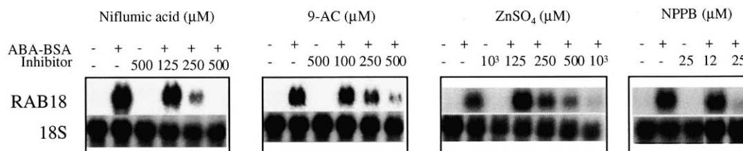
Fig. 6. Induction of RAB18 gene expression triggered by an extracellular ABA perception is mediated by anion channel activity in A. thaliana suspension cells. Northern blot analysis of total RNA (10 \mu g) from cells incubated for 3 h with ABA–BSA conjugate at 10^{-5} M equivalent ABA and anion channels blockers (zinc, niflumic acid, 9-AC and NPPB) simultaneously. Similar RNA loading was checked by hybridization with an Arabidopsis 18S ribosomal cDNA probe.
