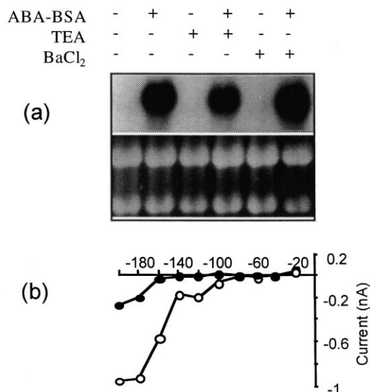
Fig. 3. Induction of RAB18 gene expression triggered by an extracellular ABA perception is independent of \text{K}^+ channel activities in A. thaliana suspension cells. a: Northern blot analysis of total RNA ( 10 \mu\text{g} ) from cells incubated simultaneously for 3 h with ABA-BSA conjugate ( 10^{-5} M equivalent ABA) and TEA-Cl ( 10 mM) or \text{BaCl}_2 ( 10 mM). Ethidium bromide staining of rRNAs is shown as control. b: Current-voltage relationship of \text{K}^+ inward currents recorded before (dark circles) and after (open circles) TEA-Cl ( 10 mM) adding. Plasma membrane currents resulting from voltage pulses from -200 to -20 mV (in 20 mV steps for 2 s). Holding potential was -40 mV. The diameter of the cell was 42 \mu\text{m} .
