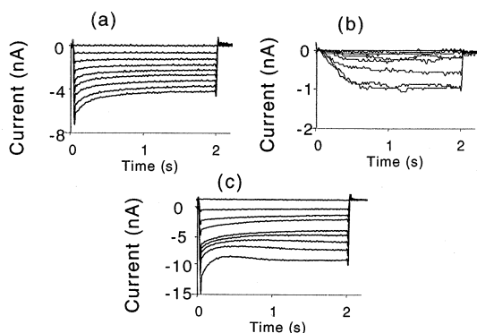
Fig. 1. Intact A. thaliana suspension cells exhibit three distinct patterns of whole-cell IRC. Currents were recorded on 4-day-old cells in fresh culture medium ( n=132 ). Plasma membrane currents resulting from hyperpolarizing voltage pulses from -200 to -40 mV for 2 s (in 20 mV steps). The holding potential was -40 mV. a: 71\% of the cells exhibit a typical anion-like current pattern. The diameter of the cell studied in this example was 42 \mu\text{m} . b: Whole-cell \text{K}^+ IRC were also well-resolved in 11\% of the cells. The diameter of the cell studied in this example was 38 \mu\text{m} . c: 18\% of the cells show a complex inward current pattern. The diameter of the cell studied in this example was 30 \mu\text{m} .
